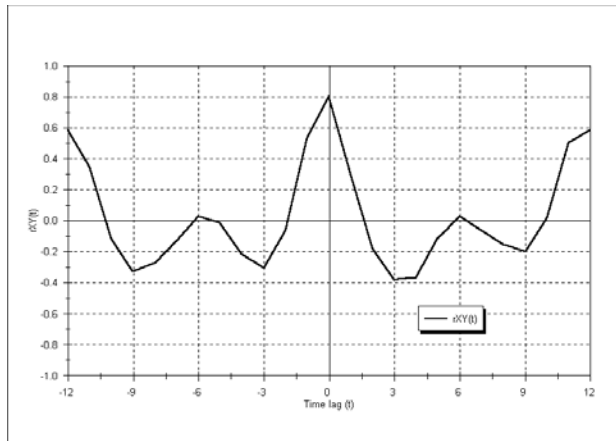
Figure 3.3: Crosscorrelogram
