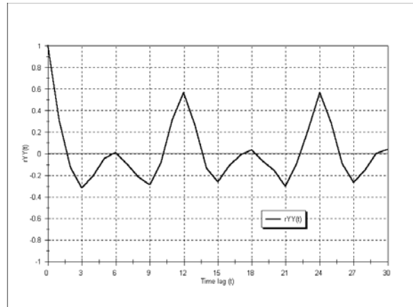
Figure 3.4: Autocorrelogram
